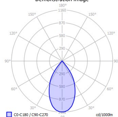
Photometric curve
